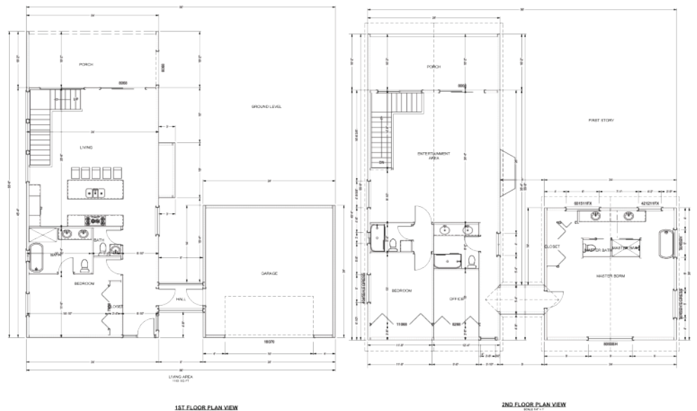
1ST FLOOR PLAN VIEW
